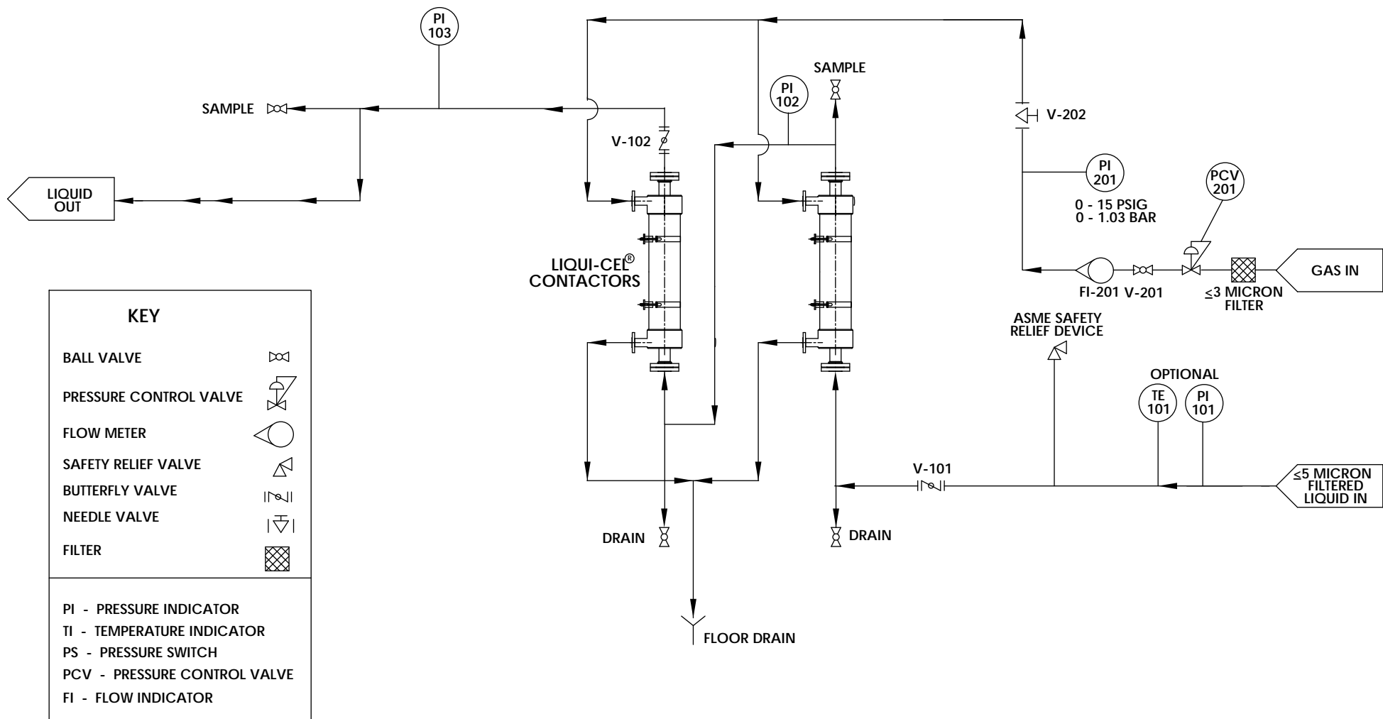
SWEEP MODE VERTICAL USING COMPRESSED GAS SOURCE
